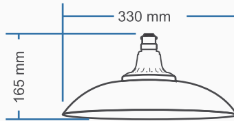
SKYLIGHT - 20W
