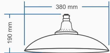
SKYLIGHT - 25W
