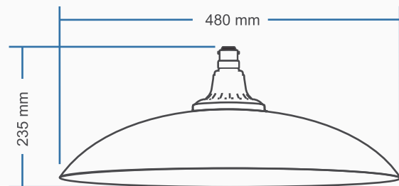
SKYLIGHT - 40W
