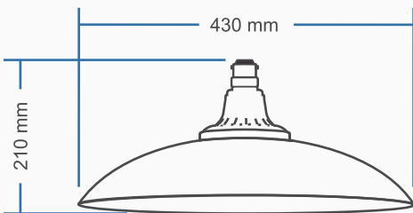
SKYLIGHT - 30W
